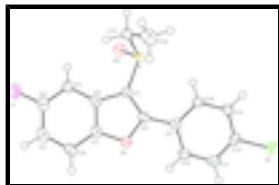
Fig. 1. The molecular structure of the title compound with the atom numbering scheme. Displacement ellipsoids are drawn at the 50 % probability level. H atoms are presented as small spheres of arbitrary radius.
