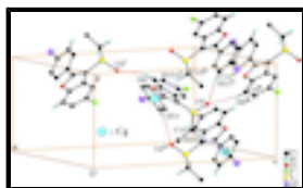
Fig. 2. C—H...O and C—H... \pi interactions (dotted lines) in the crystal structure of the title compound. Cg denotes the ring centroid. [Symmetry codes: (i) x, -y + 3/2, z - 1/2 ; (ii) -x + 1, y - 1/2, -z + 3/2 ; (iii) x, -y + 3/2, z + 1/2 ; (iv) -x + 1, y + 1/2, -z + 3/2 .]
